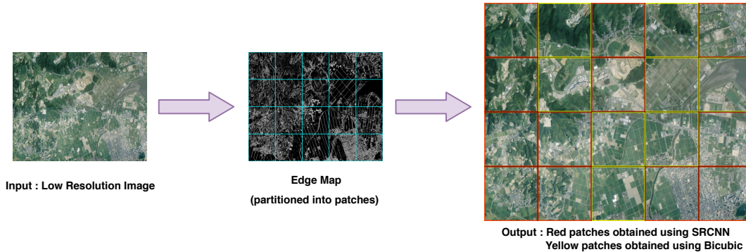
Figure 3. Demonstration of qualitative results obtained using our selective deep super-resolution approach on a given low resolution image.
