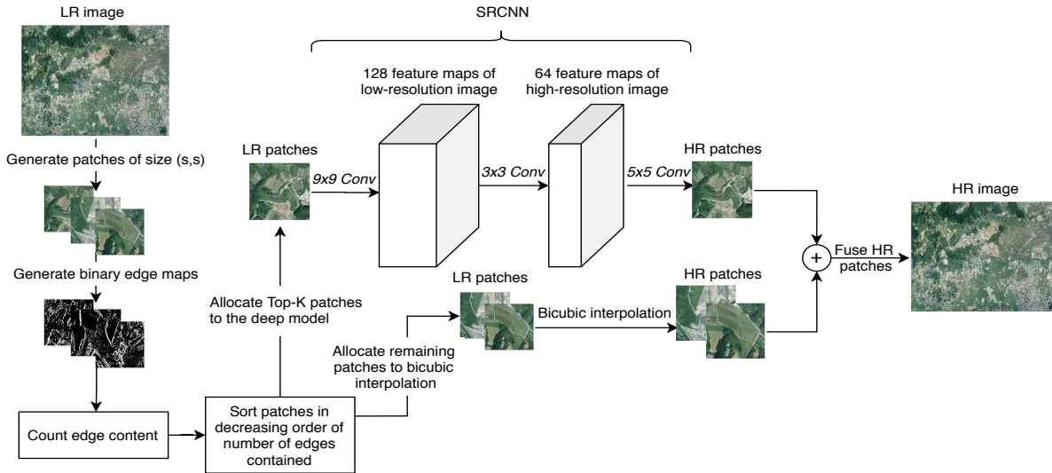
Figure 1. Proposed Method: The low-resolution image is divided into patches, and edge maps are generated where the top k patches (descending order) based on edge content are allocated to the deep model, and the remaining patches are allocated to bicubic interpolation. Finally the high-resolution patches obtained from the deep and non-deep methods are fused to obtain the output image
