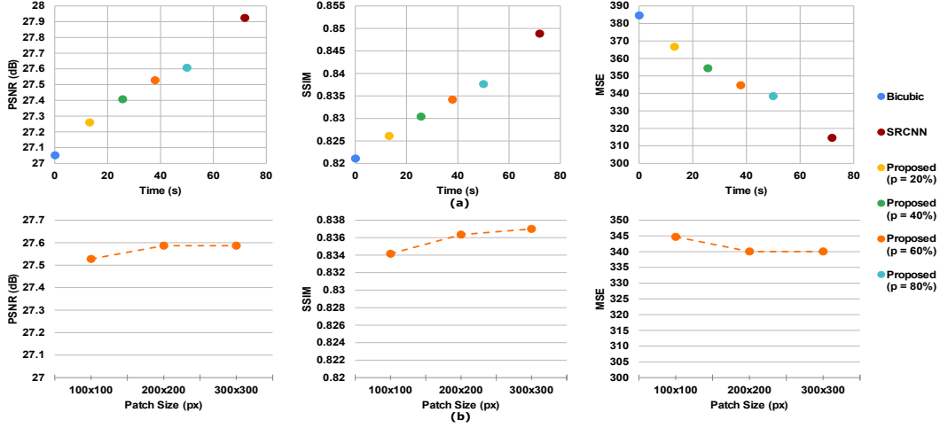
Figure 2. Ablation Study: (a) Scatter Plot describing the variation in the performance of Bicubic Interpolation, SRCNN and Proposed Method over time taken for super-resolution for a fixed patch size of 100 \times 100 (b) The performance of the Proposed Method on different evaluation metrics over several choices of patch size.
